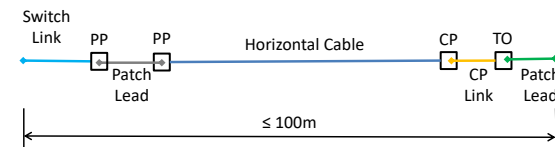
Diagram 4: Cross-connect – CP – TO
