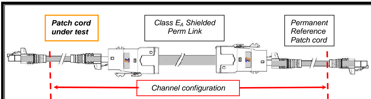
Figure 2: Test set up - Channel configuration
