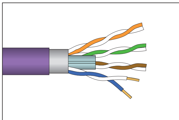
CA120DCA - Category 6 F/UTP Shielded Cable - Dca
