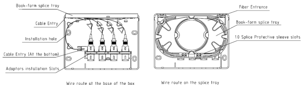
Pic1: The fiber route schematic diagram
