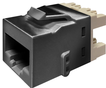
KJ Series Keystone Modular Jack, 8-position, category 6, unshielded UTP, black
