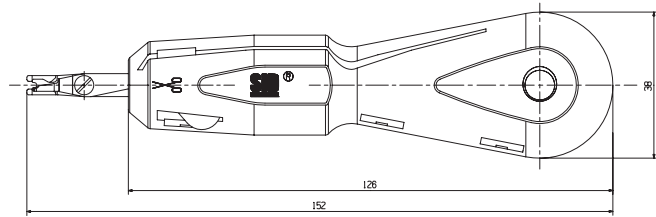
Dimensions of SID comfort tool
